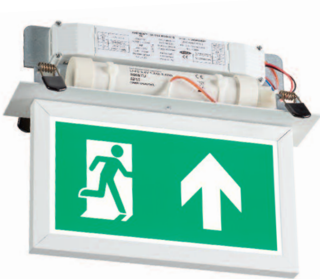
ME/RECE/DALI/WH showing integral proSeries LM1M24 and BO68/TU LiFePO4 battery
